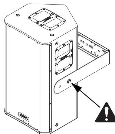
Figure 5- Yoke behind enclosure.
